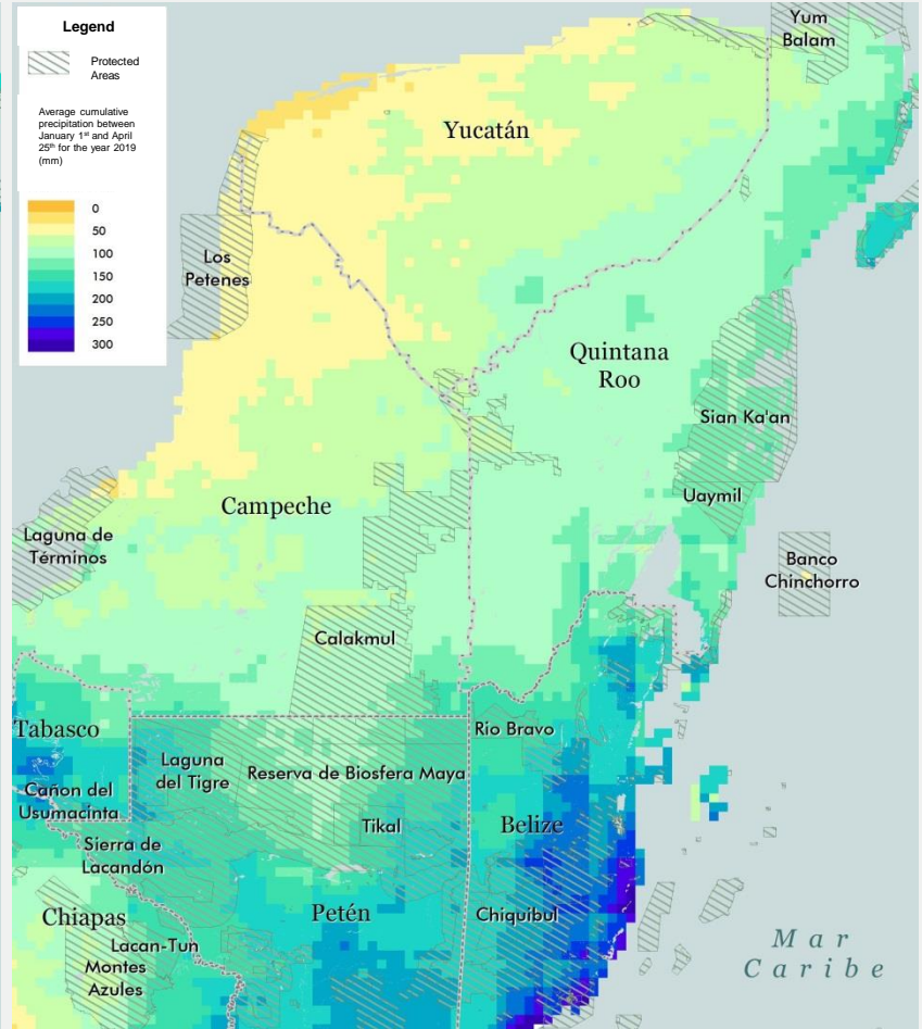
Cumulative precipitation between January 1st and April 25th, 2019
