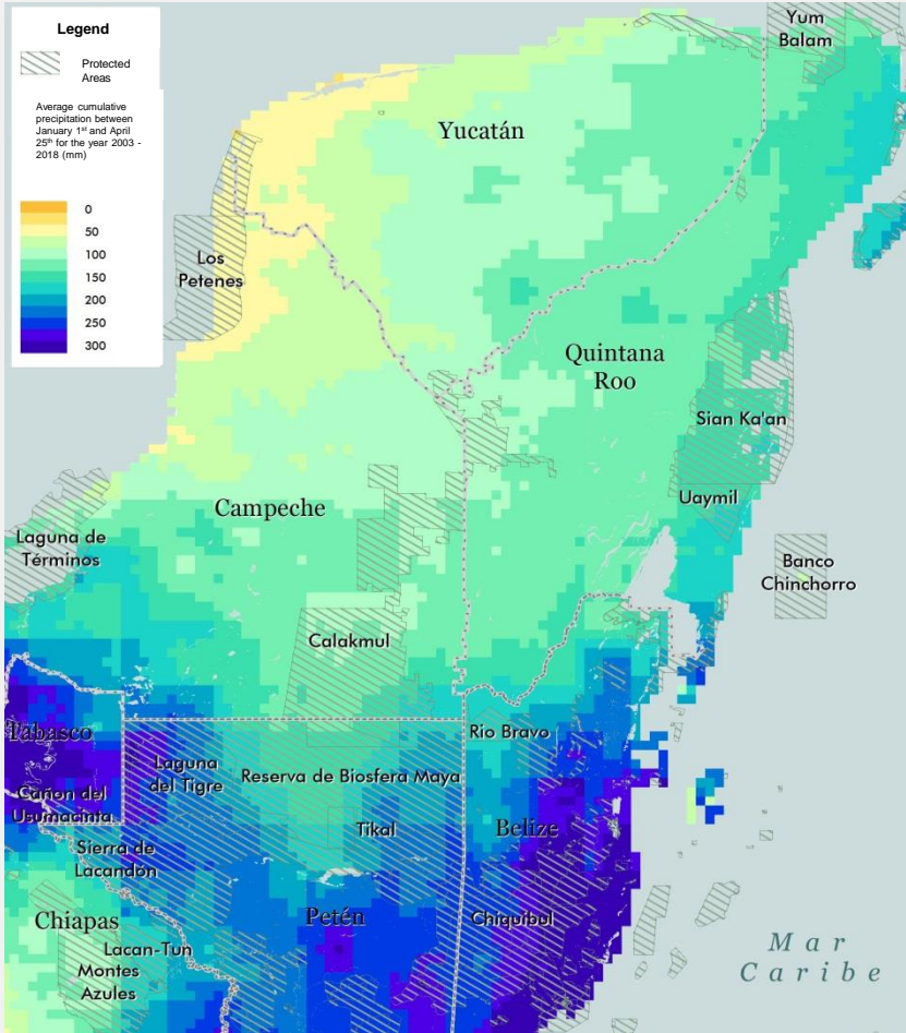
Average cumulative precipitation 2003-2018 between January 1st and April 25th
